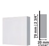
Roseta 175 | Rosette | Roseta 70 x 70 x 20mm 2 3/4" x 2 3/4" x 13/16" Cód. | Code - 24347
